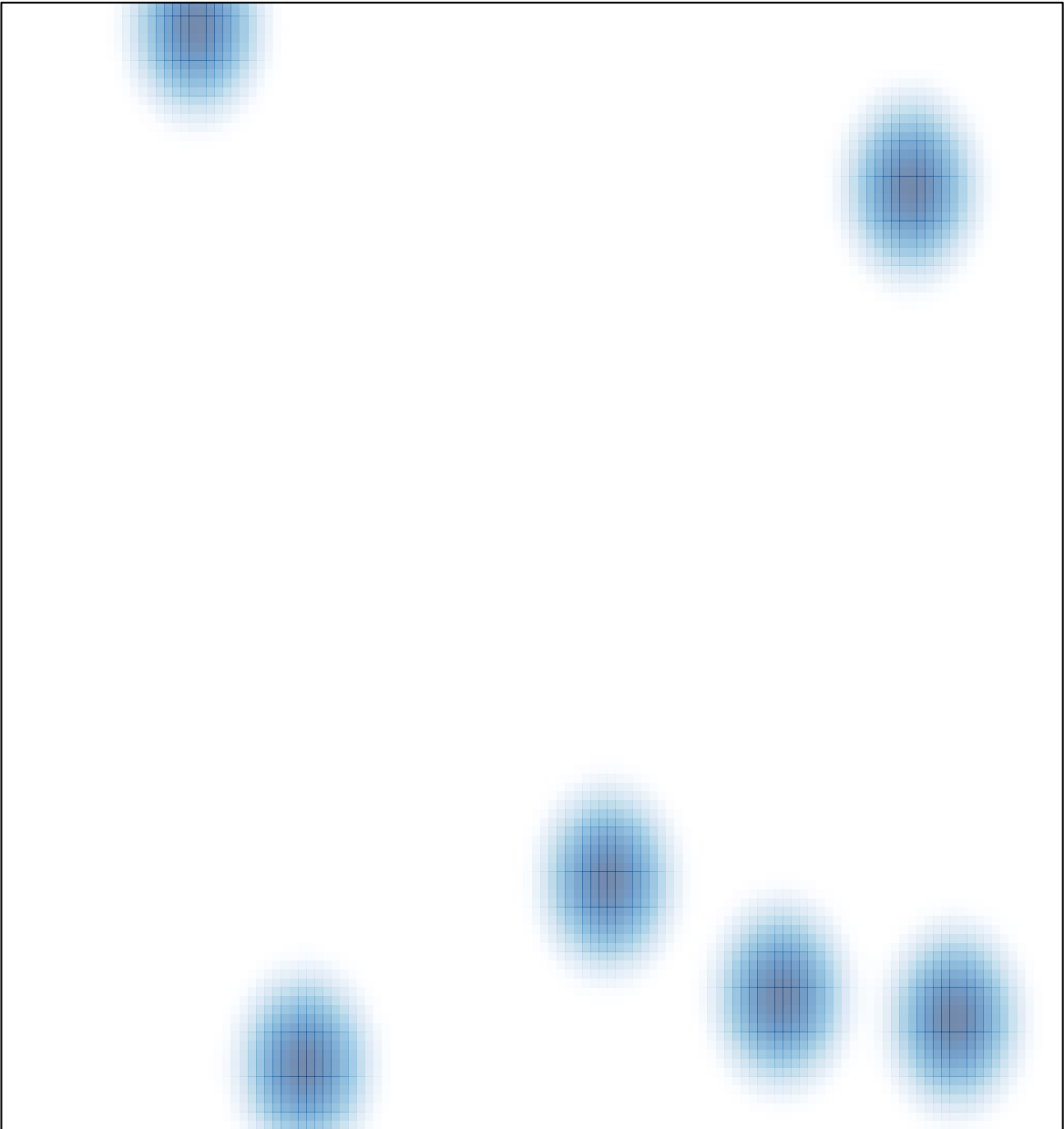
# features = 6 , max = 1
